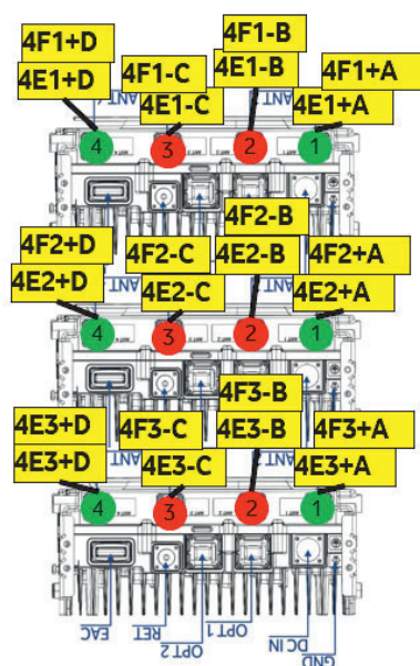
RRH Dual Band 1800/2100
